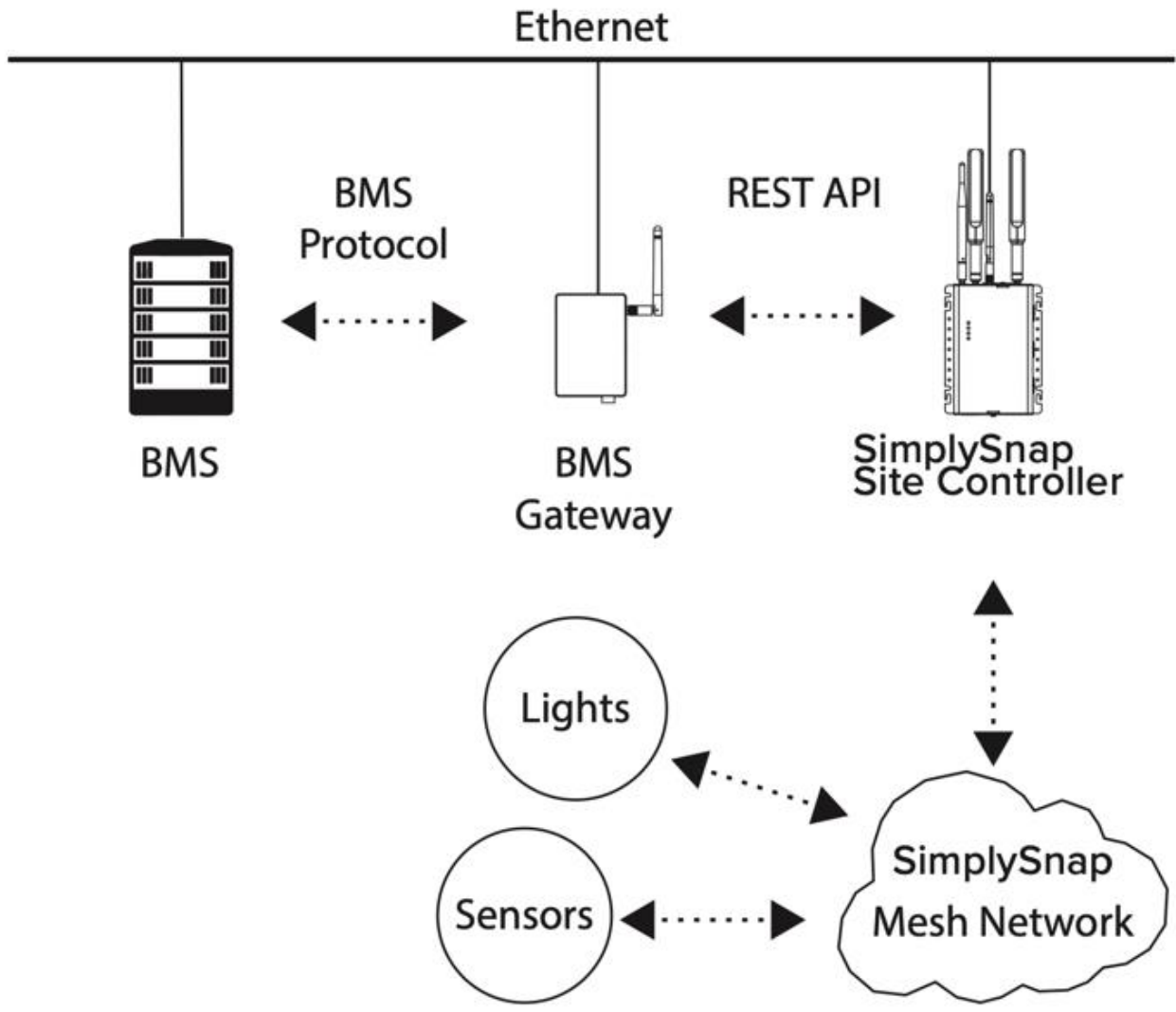
Example Setup of a BMS/SimplySnap Integration
