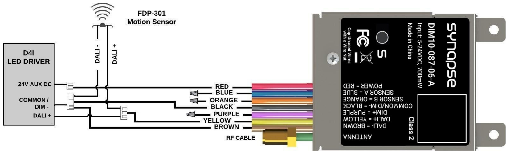
Figure 4 - DALI-2 Wiring Diagram
