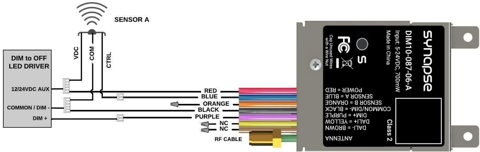
Figure 3 - DIM to OFF Wiring Diagram
