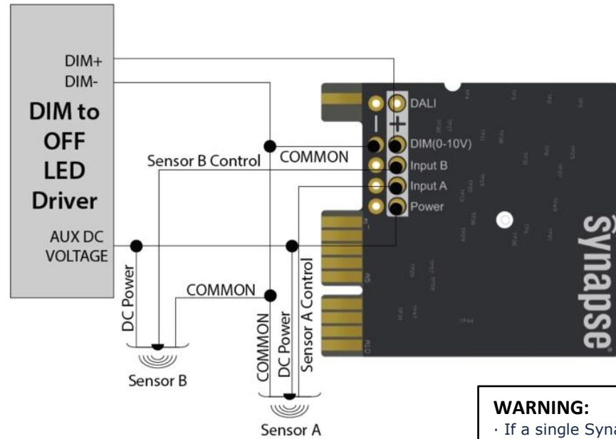
Figure 2 – Dim to OFF Wiring Diagram
