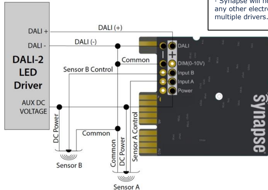
Figure 3 – DALI-2 Wiring Diagram
