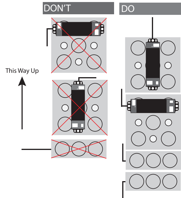
FIGURE 1 - ANTENNA ORIENTATION
