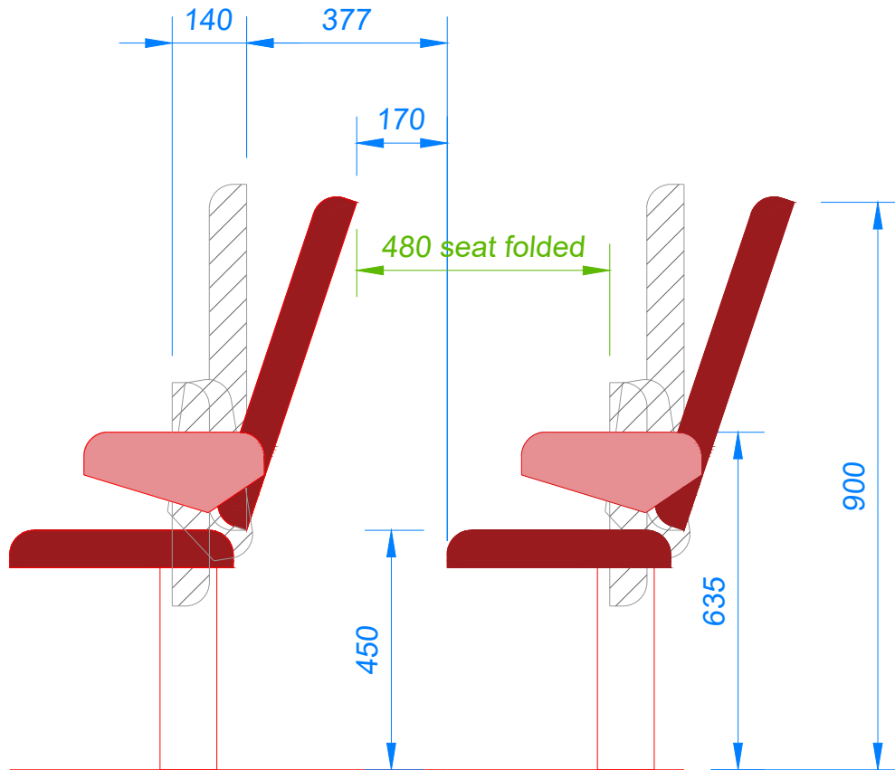
SIDE ELEVATION
