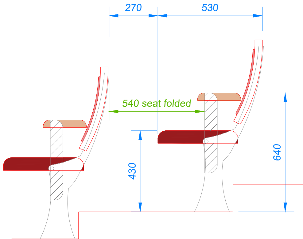
SIDE ELEVATION
