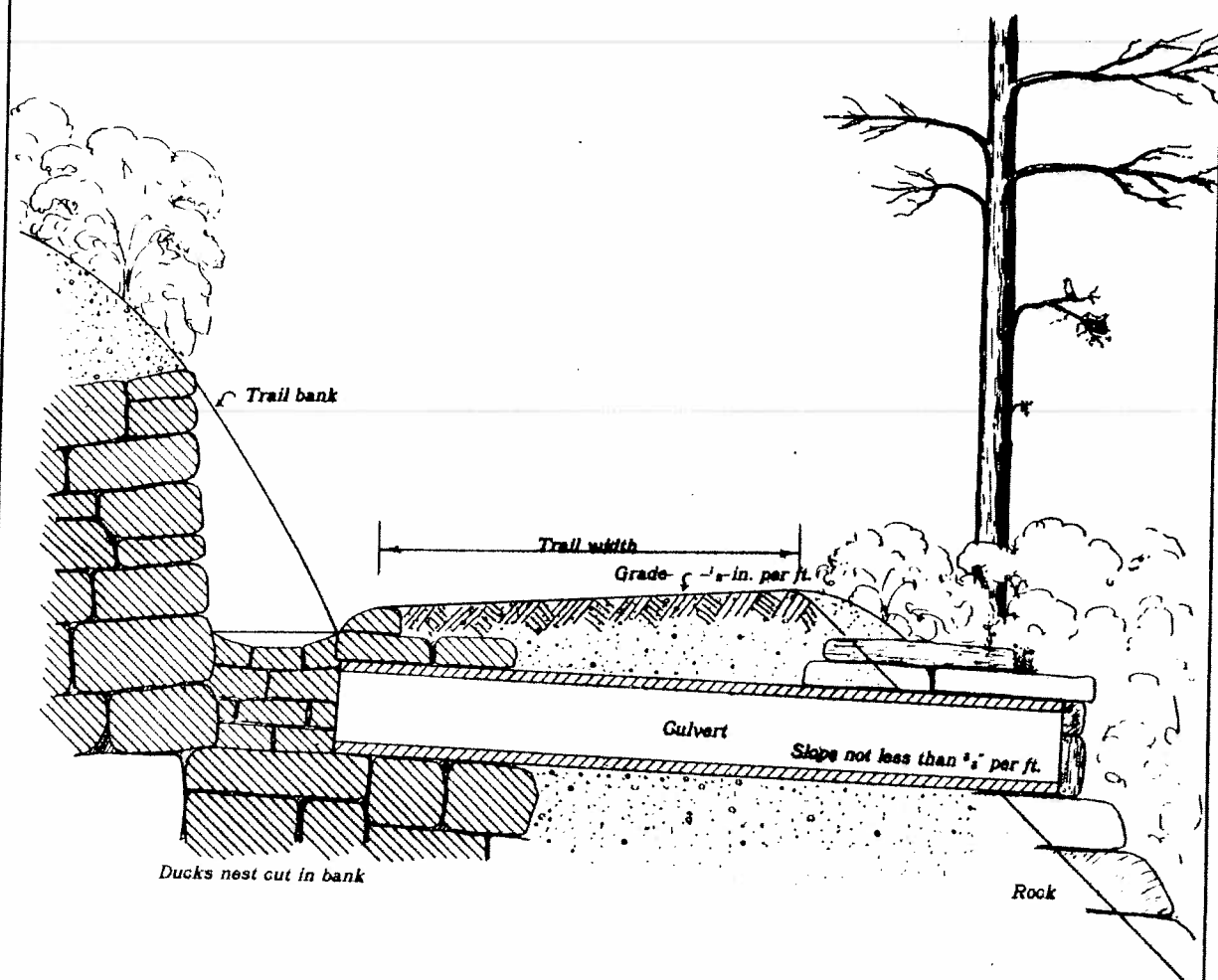
DRAINAGE TO INSIDE OF TRAIL SKETCH NO. 21
