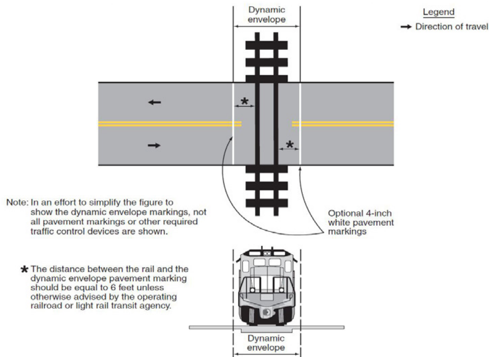
Figure 19. Example of Dynamic Envelopement Pavement Markings at Grade Crossings
