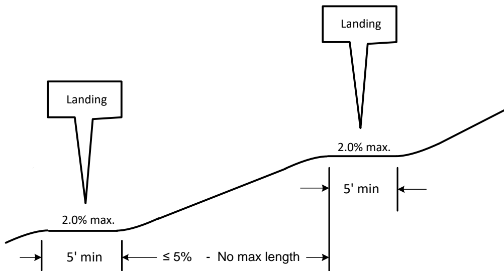
Exhibit 1515 - 6 Shared-Use Path Landing Profile
