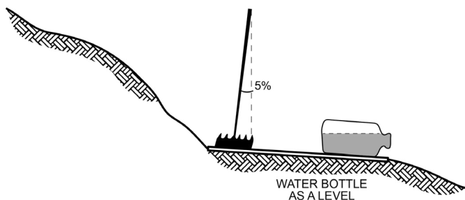
Figure 6–14. The outslope of 3–8 percent should be barely detectable to the eye. A partially filled water bottle makes a good level, or you can stand a McLeod on the trail tread—the handle should lean downhill.
