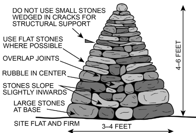
CAIRN VERTICAL SECTION
