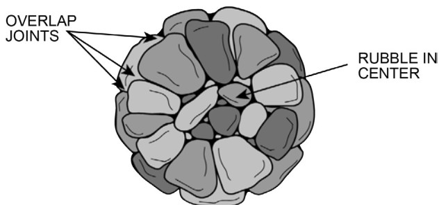
CAIRN HORIZONTAL CROSS SECTION
