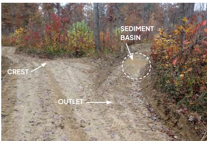
Figure 4–3. A sediment basin connected to a rolling grade dip catches eroded material that can be reused in routine trail maintenance. Consider increasing the number of rolling dips if the sediment basin fills in less than 3 years. Daniel Boone National Forest, Kentucky. USDA photo by Matt Able.
