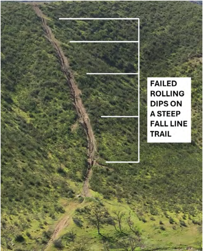
Figure 2–23. Heavily eroded fall line trail with several failed rolling dips. Mendocino National Forest, California. USDA photo by Scott Johnson.
