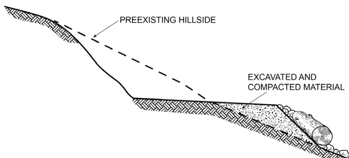
Figure 6–10. The tread on a partial-bench trail is part hillside and part fill material and is outsloped at least 5 percent. This technique is less desirable than the full-bench construction technique, as uncompacted fill will more easily erode and cause the trail to narrow over time. Diagram based on Forest Service standard trail drawing STD 911–01 (B section).
