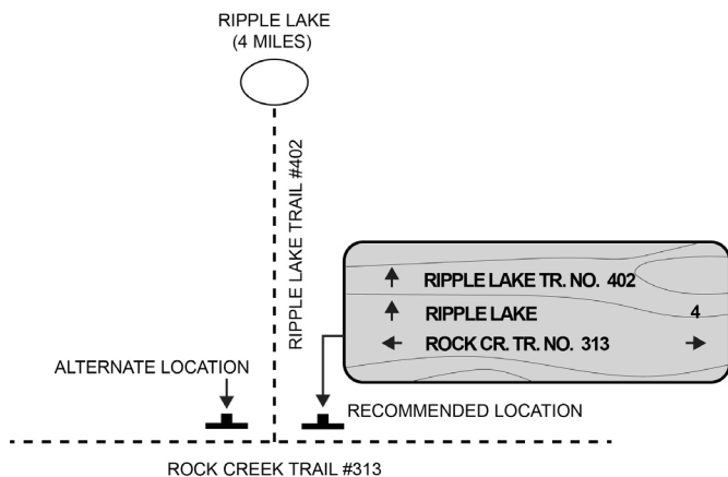
Figure 5–3. Sign placement example on a trail not designated for motor vehicle use.
