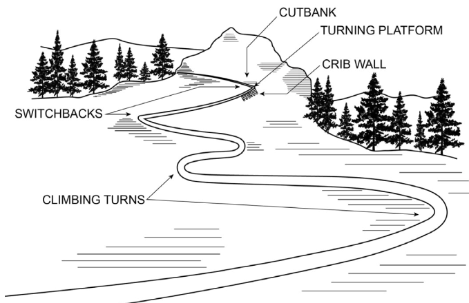
Figure 4–28. Climbing turns should be built on moderate slopes (less than 25 percent), whereas switchbacks can be constructed on steeper grades. Switchbacks require more technical construction techniques, such as installing crib walls.
