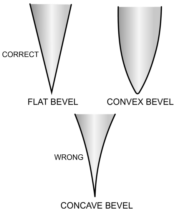
Figure 7–23. Illustration of correct and incorrect blade bevels.
