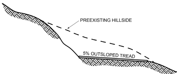
Figure 6–9. Construct a full-bench trail by cutting the full width of the tread into the hillside. Outslope the tread 3–8 percent (or maximum 5 percent on trails designed for accessibility). Diagram based on Forest Service standard trail drawing STD 911–01 (A section).
