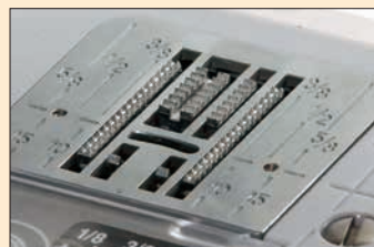
7-Point Feed Dog
