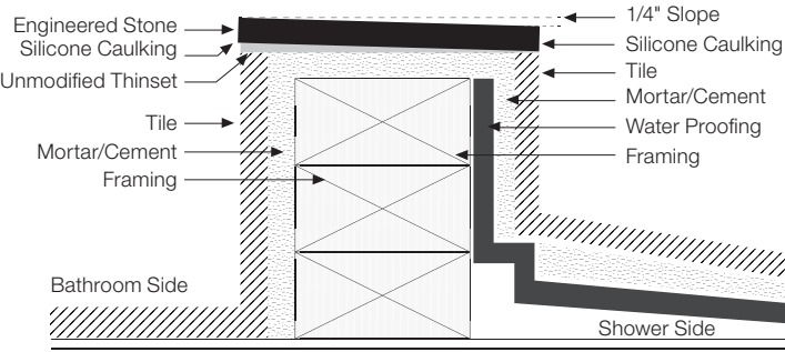
Installation Diagram
