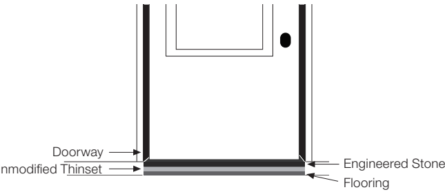
Installation Diagram
