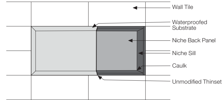
Installation Diagram
