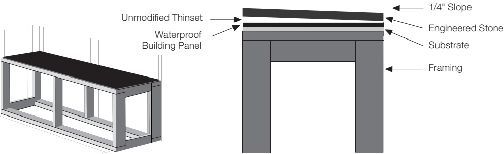
Installation Diagram
