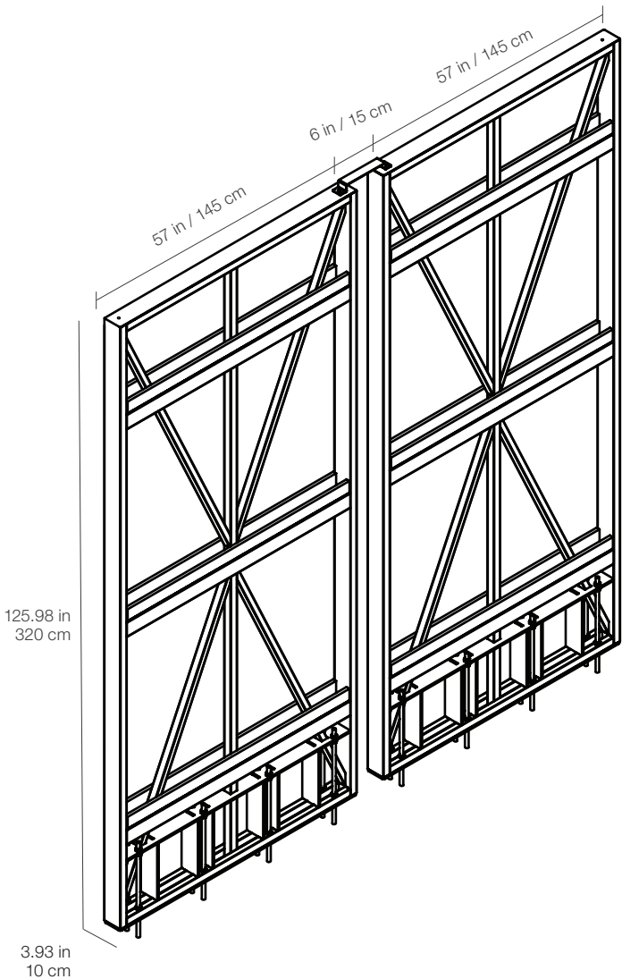
Frame structure spacing between two panels for side-by-side installation
