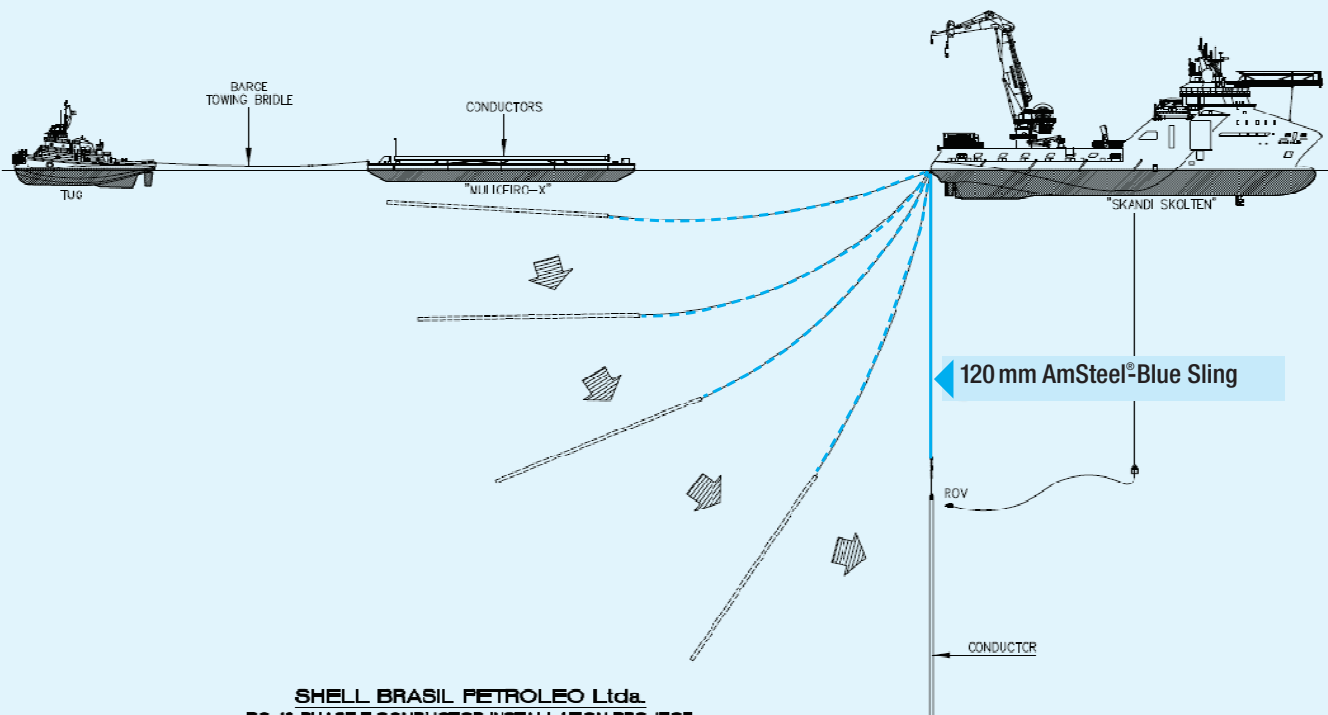
120 mm AmSteel®Blue sling supporting the load
