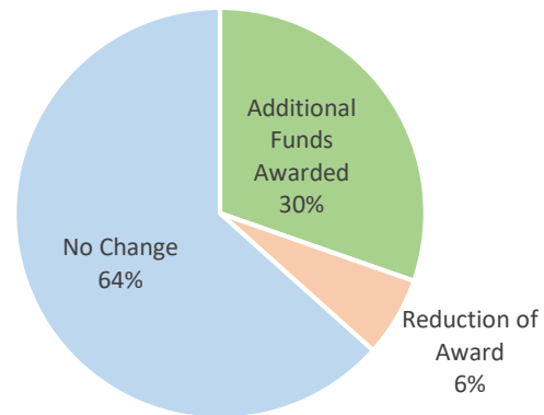
Figure 1: Award Appeals
