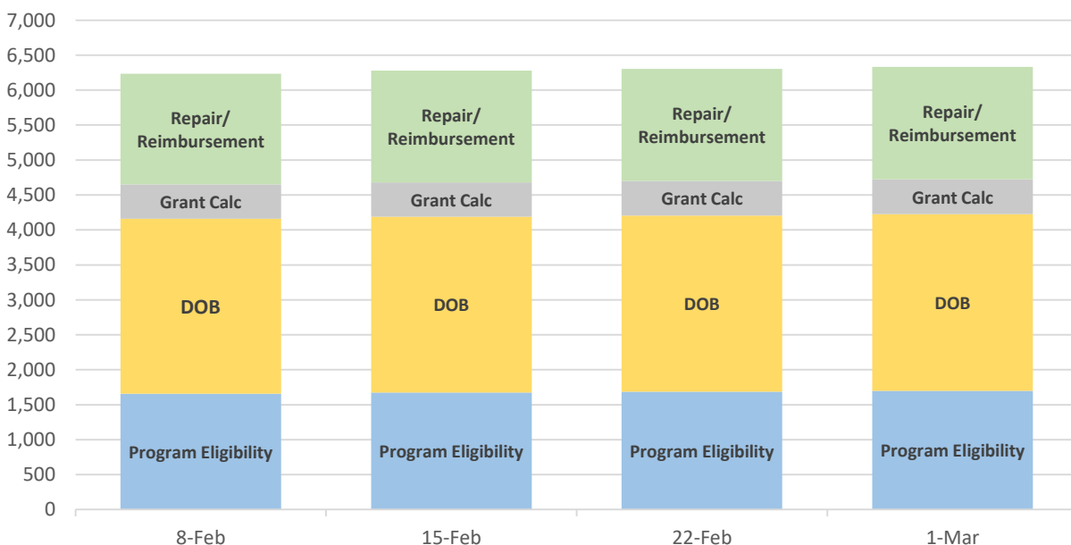
Figure 2: Reason Codes
