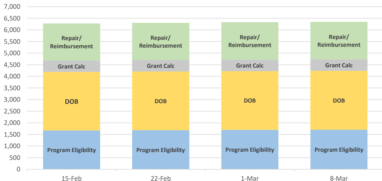
Figure 2: Reason Codes
