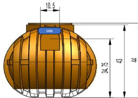
Outlet Side
