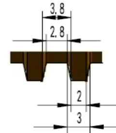
Rib Detail
