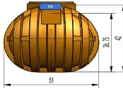
Inlet Side
