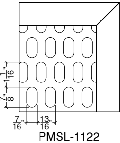
SECTION VIEW
