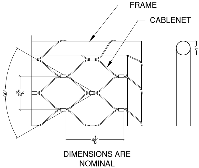
7x7 CONSTRUCTION CABLE
