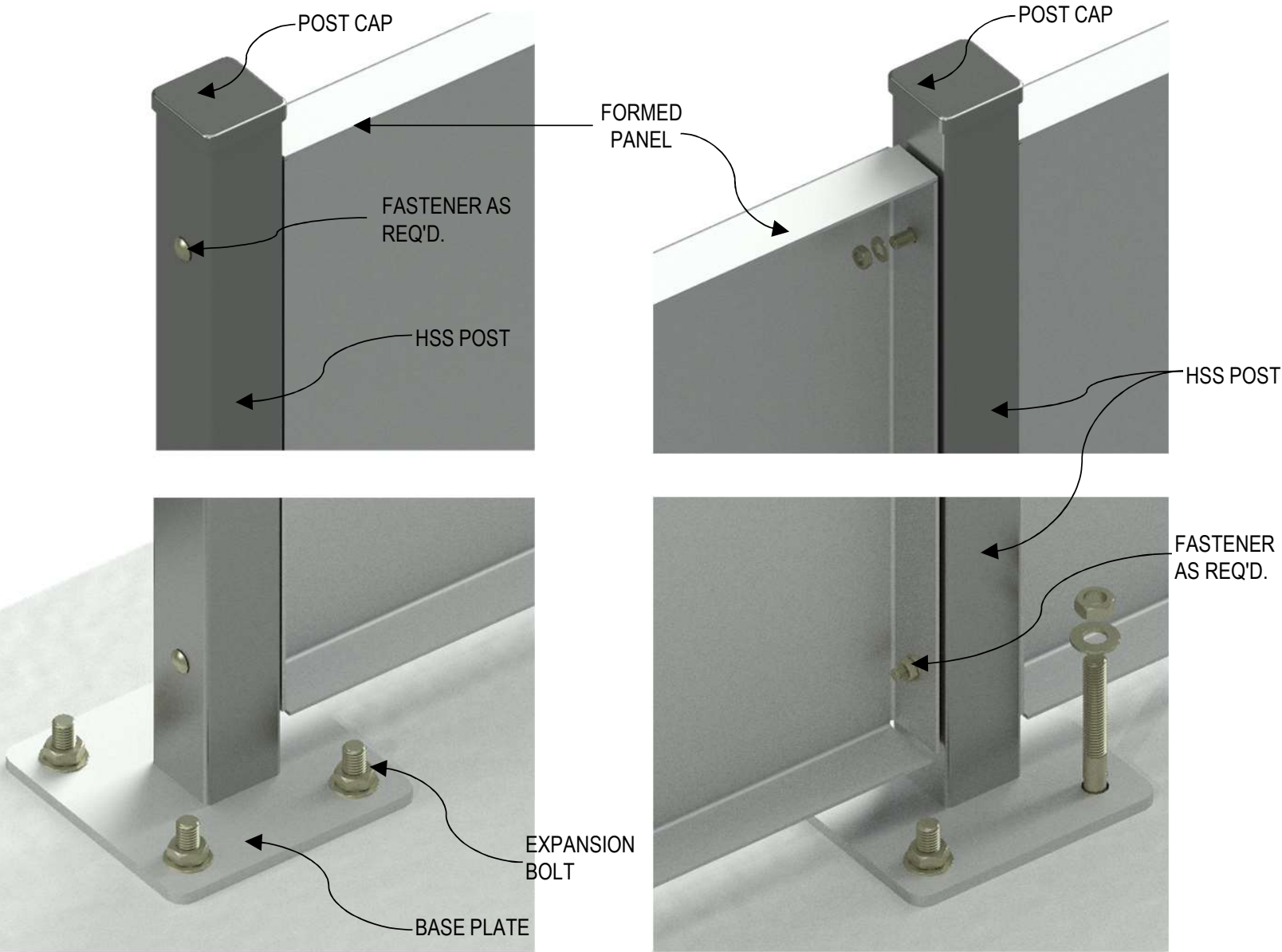
TYPICAL RENDERED DETAIL
