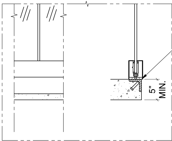
Welded @ Embed Angle - $$$
