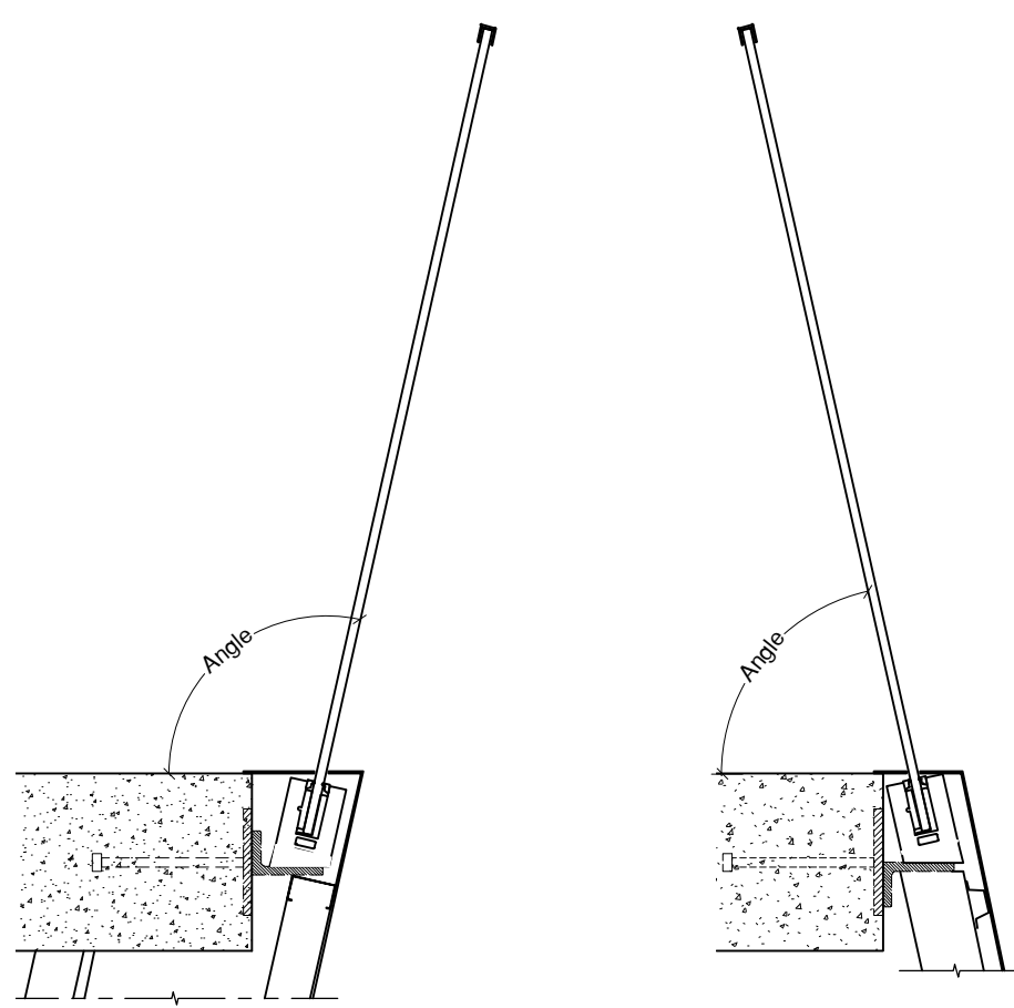
Obtuse Angle Tilt Shoe
