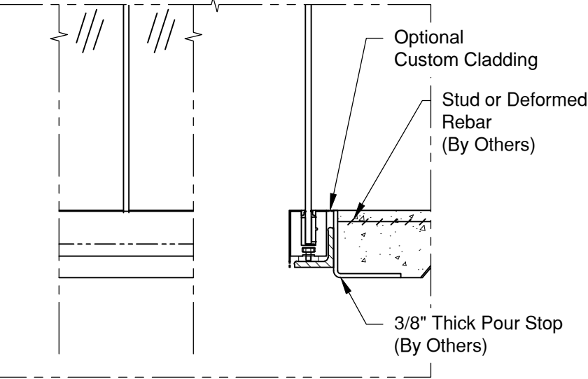
Welded @ Steel Angle - $$
