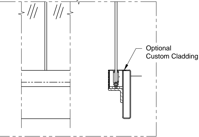
Welded @ Steel Angle Welded @ Steel Tube - $$
