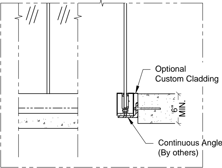
Welded @ Steel Angle Anchored @ Concrete - $$
