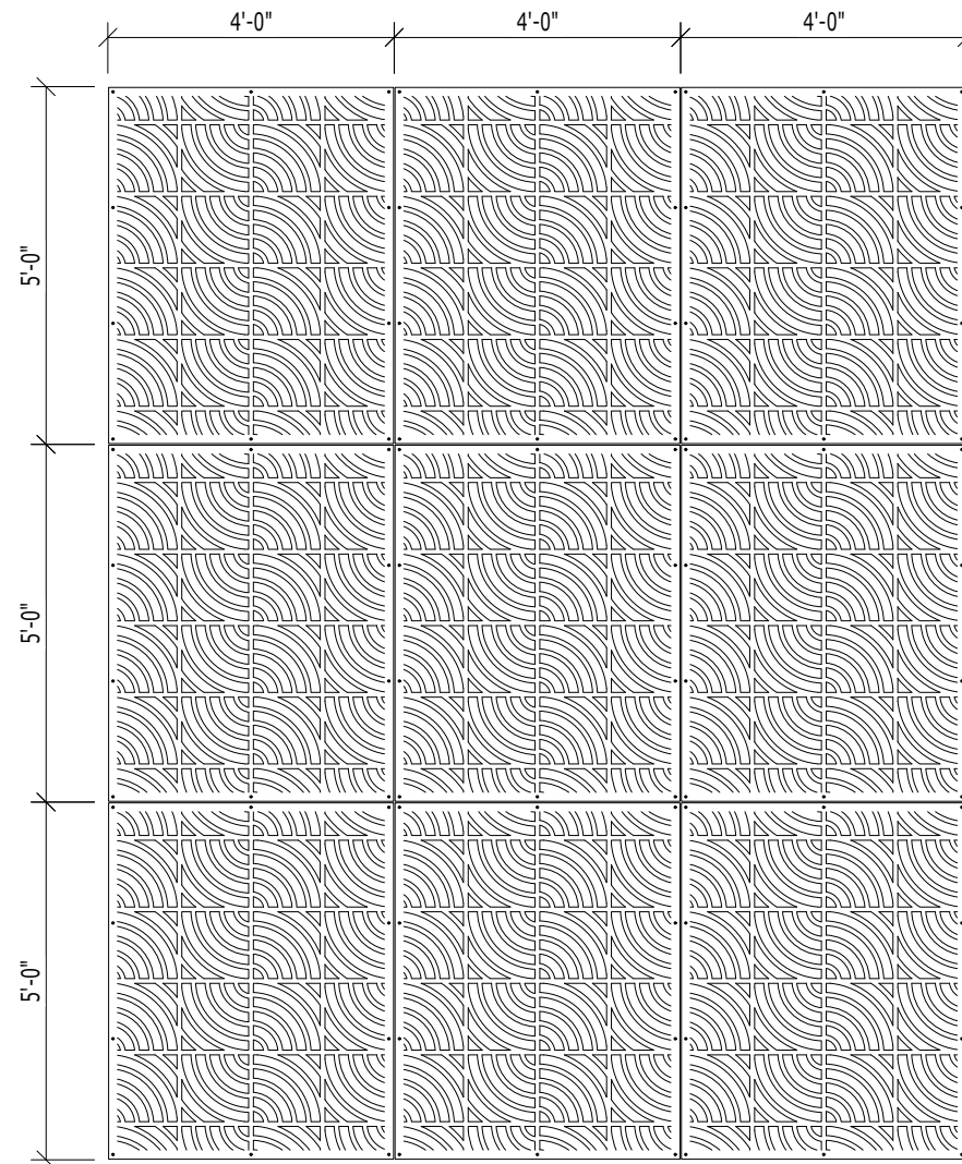
WALL SYSTEM WITH 4'-0" x 5'-0" STANDARD PANELS
